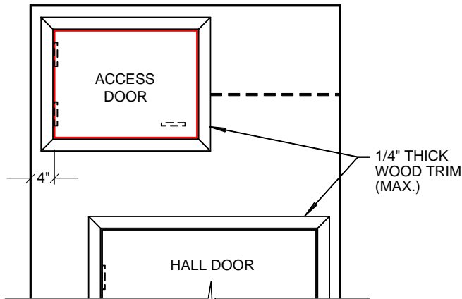
ELEVATION VIEW 'B'
