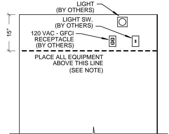
ELEVATION VIEW 'C'
