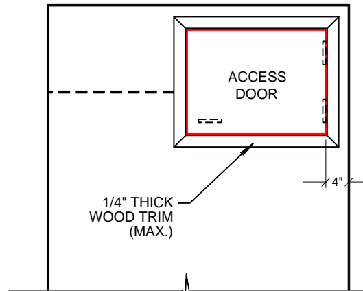
ELEVATION VIEW 'B'
